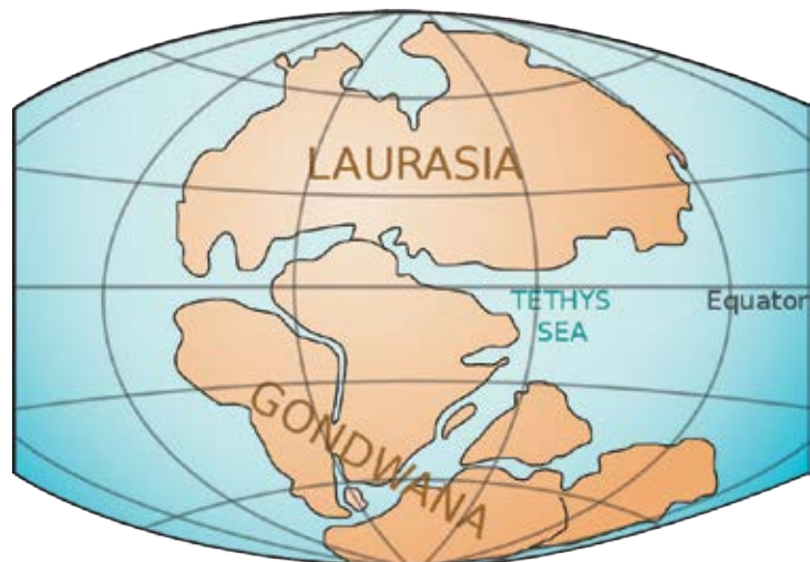
Fig. 7. Gondwana – the last known supercontinent in the Earth's history.
