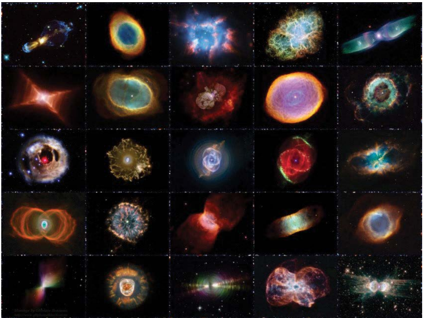
Fig. 13. A gallery of planetary nebulae within the Milky Way. Each image in this gallery represents the death of a low mass star like the Sun. The ring like structure is gas that was once part of the star and is now pushed out in a slow outburst. At the center of each planetary nebula is the white dwarf.
