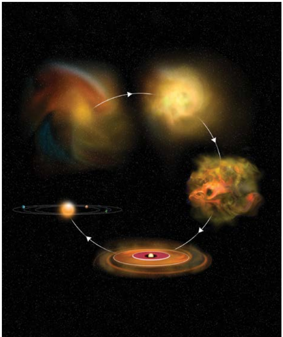
Fig. 7. The sequence of steps that leads to the birth of a star. Inside a cold dense cloud of gas, a fragmented region starts collapsing under its own gravity. The collapse continues until a star forms at its centre, along with planets around it. A star is born when the temperature at the central region of the collapsing fragment equals 10 million Kelvin, and the density approximately 160 gms/cc (about 10 times the density of lead).
