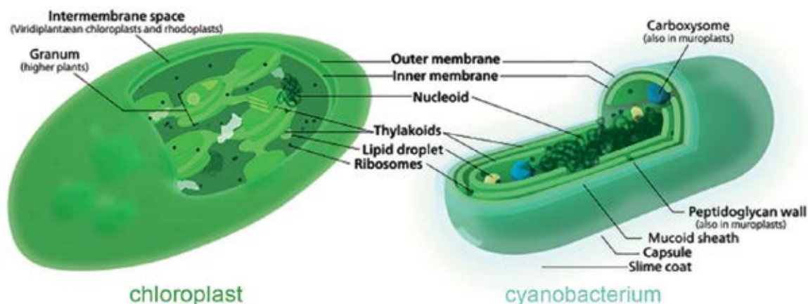
Fig. 2. Margulis's endosymbiotic theory was influenced by the botanist Mereschkowsky's comparison of similarities between chloroplasts and cyanobacteria.
